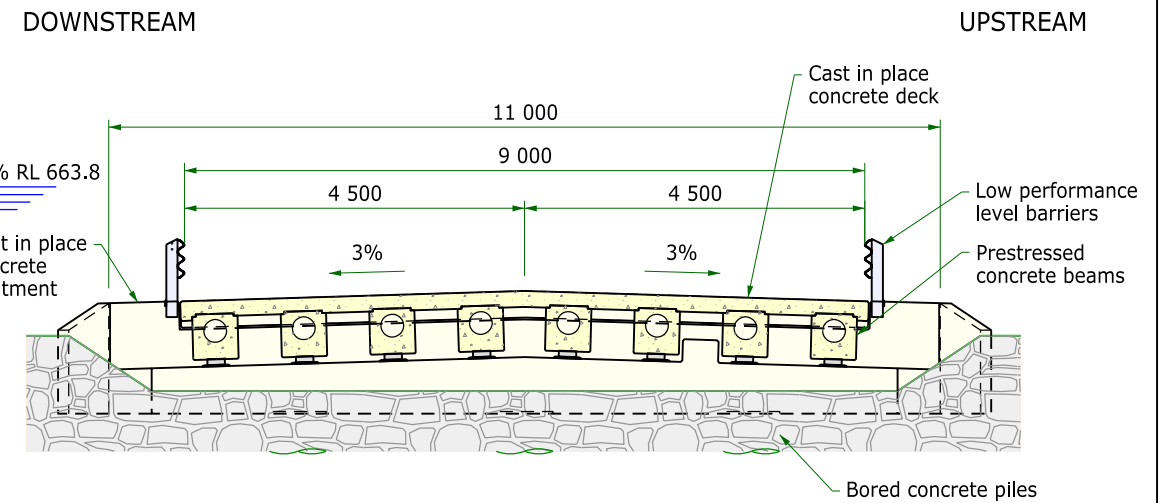
SECTION 1 1:100
