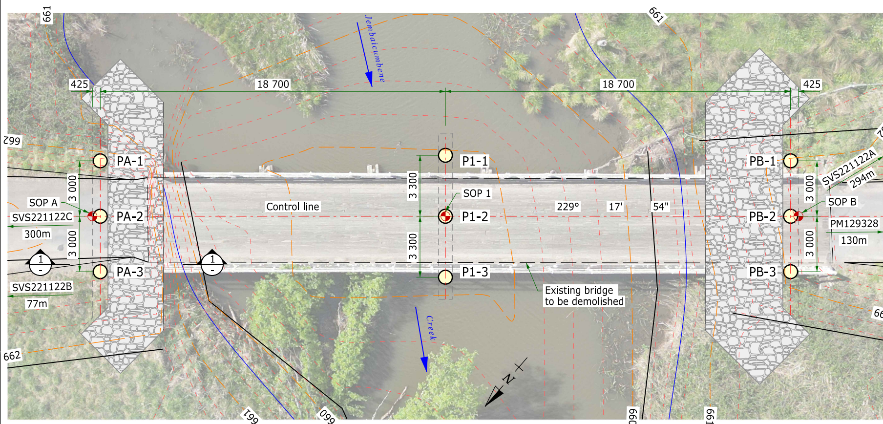
PLAN 1:200
